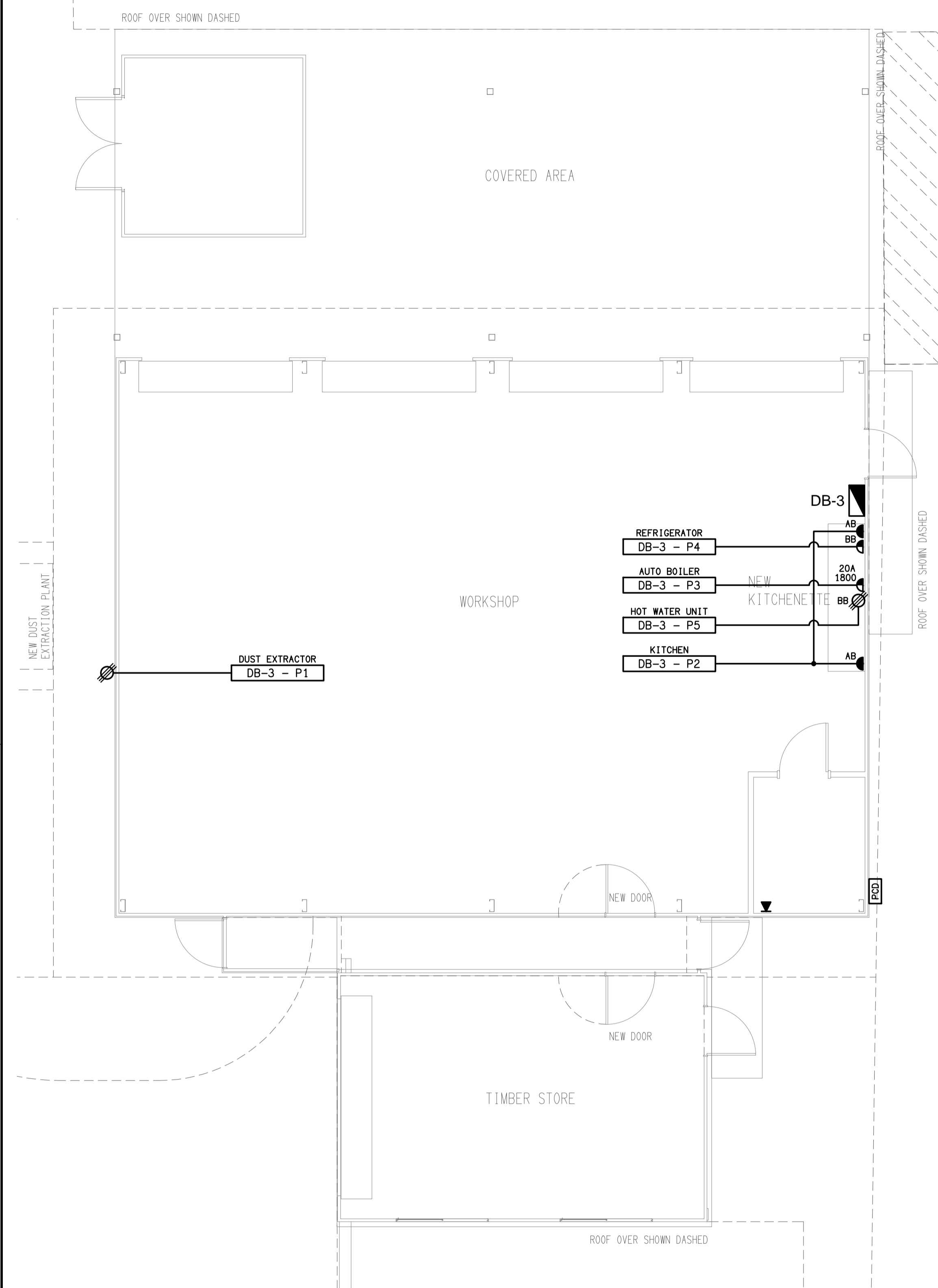
BUILDING 3 FLOOR / REFLECTED CEILING PLAN SCALE 1:50
